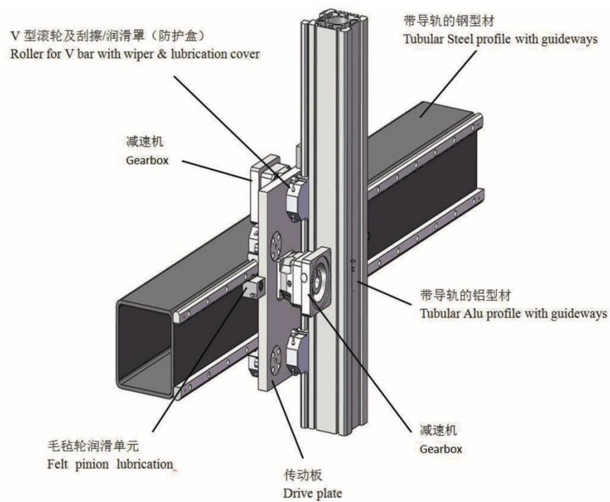
V型导轨齿条传动系统 (中载荷) Guideway V Rack Drive Systems (Medium Duty)
